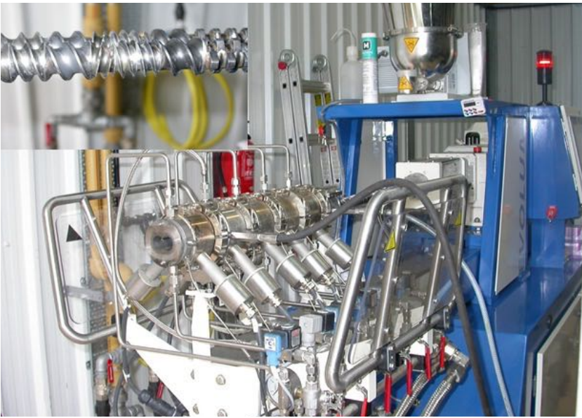
Figure 1. Twin-screw extrusion equipment at CIEMAT facilities and detail of screw configuration inside the barrels.
